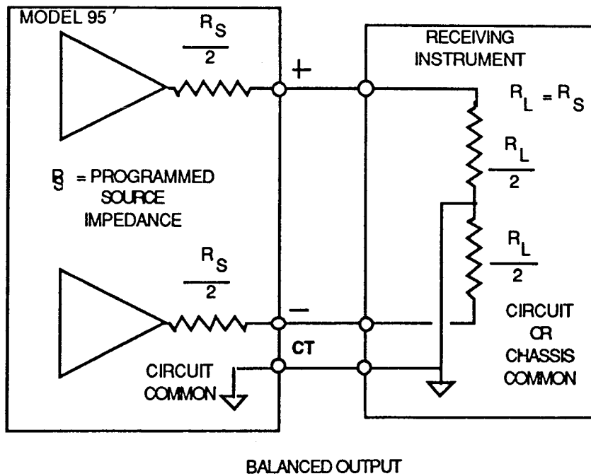
Figure 3-7. Output Terminations
