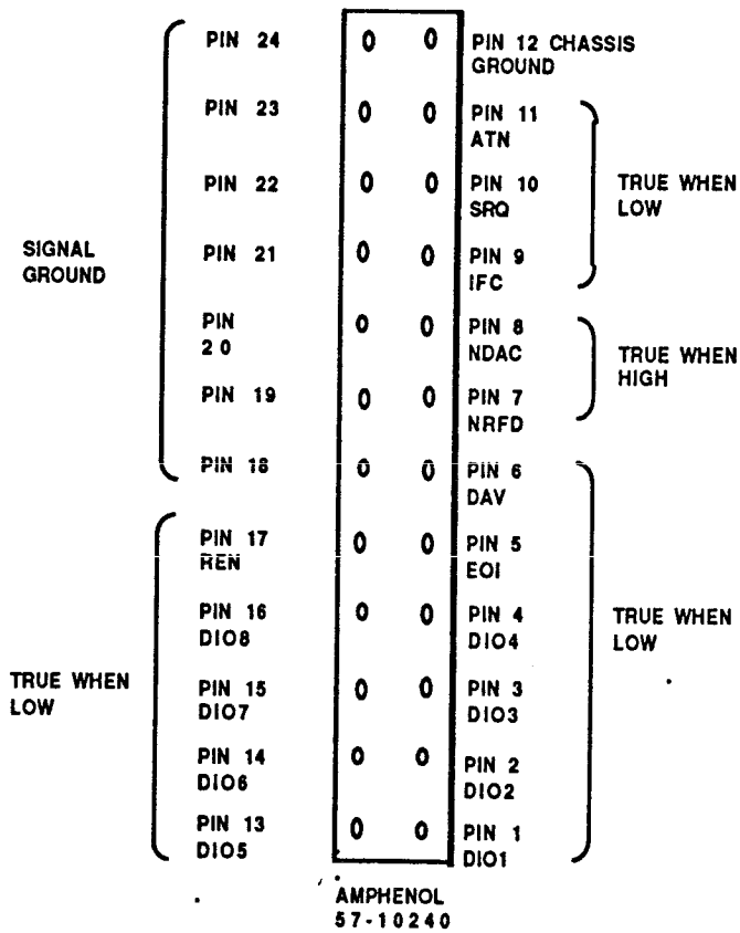
Figure 3-3. GPIB Wiring Connector Pinout
