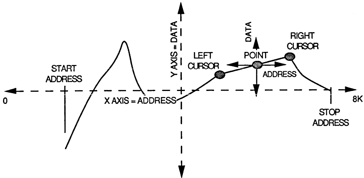
Figure 3-9 Point. 3 Point Edit
