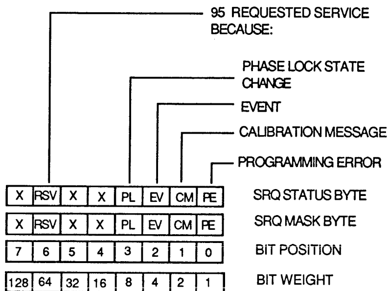
Figure 3-9. Model 95 Status Byte and SRQ Mask
