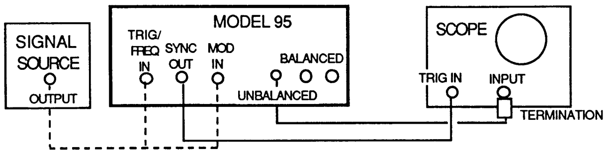
Figure 2-2. Function Checkout Interconnection
