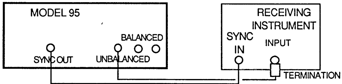
Figure 3-8. Continuous Operation Interconnection
